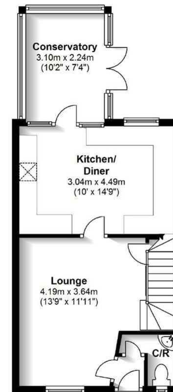
Ground Floor Approx. 40.6 sq. metres (437.3 sq. feet)
